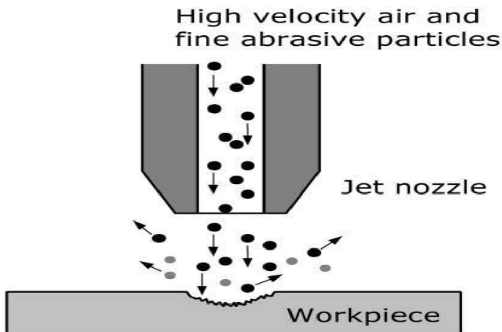
Fig.1.1 Principle of the AJM process [7]
