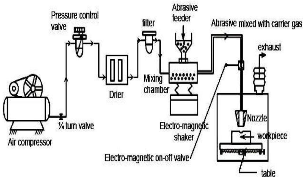
Fig.1.2 Schematic layout of AJM [25]
