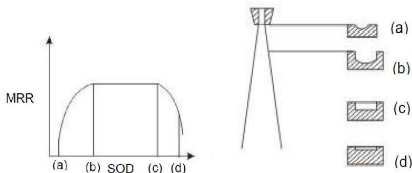
Fig.1.6 Effect of Standoff distance on MRR [26]
